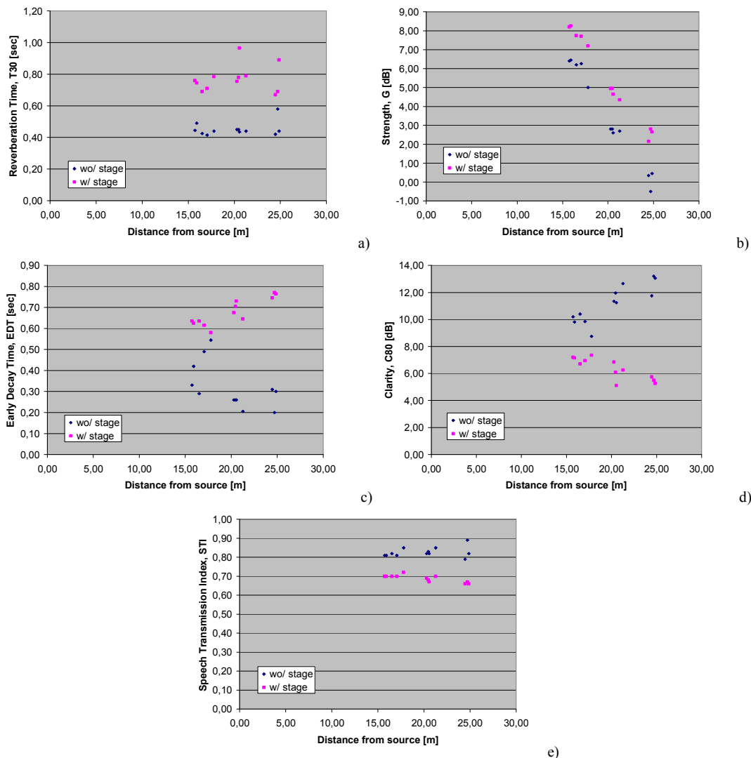
Figure 6 – T30, G, EDT, C80, STI vs distance at the Theatre of Ancient Epidauros. The source is positioned in the center of the orchestra . Each point represents the average of the values at 500Hz and 1000Hz octave bands, for the specific receiver position. The pink and blue dots indicate values obtained from the model of the theatre with and without stage, respectively.
