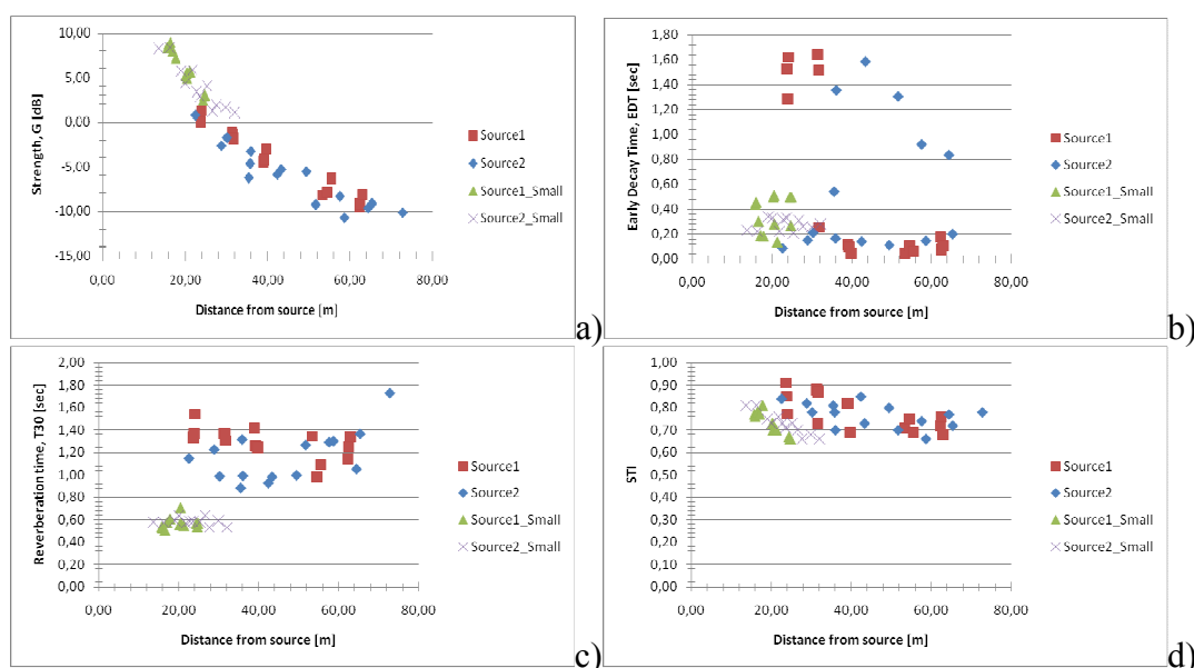
Figure 3 - G, EDT, T30 and STI versus distance in both theatres. Each point represents the average of the measured values at 500Hz and 1000Hz octave bands, for the specific source-receiver setup. The red and blue markers correspond to measurements at the Theatre of Epidaurus, while the green and purple correspond to measurements at the Theatre of Ancient Epidaurus
