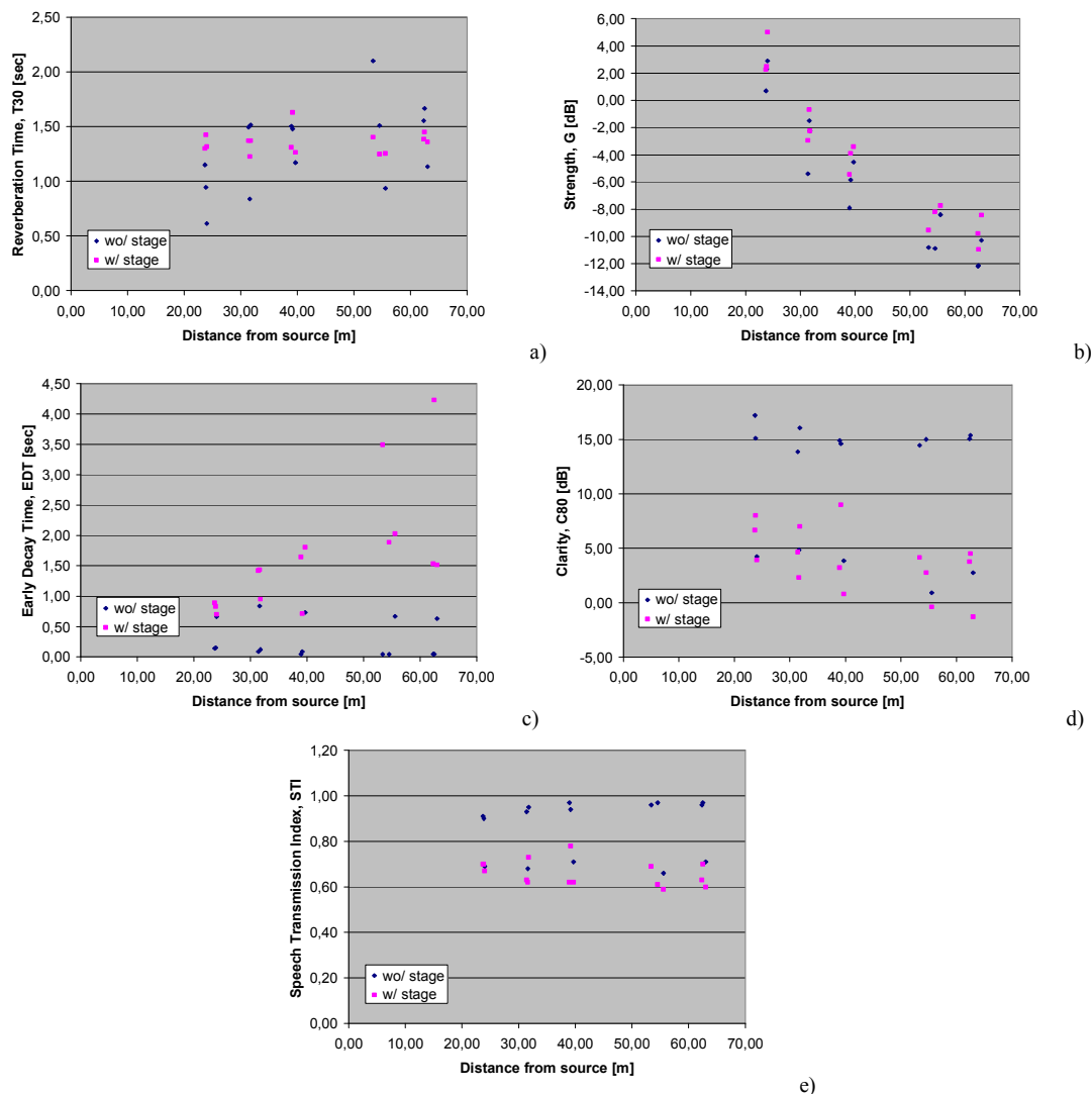
Figure 5 – T30, G, EDT, C80, STI vs distance at the Theatre of Epidauros. The source is positioned in the center of the orchestra . Each point represents the average of the values at 500Hz and 1000Hz octave bands, for the specific receiver position. The pink and blue dots indicate values obtained from the model of the theatre with and without stage, respectively.
